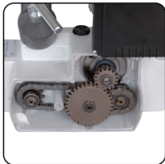
Chain drive
