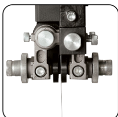
Upper and lower roller blade guide
