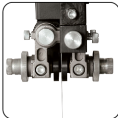
Upper and lower roller blade guide
