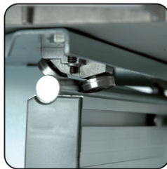
Tenoning carriage with ball-bearing sliding system
