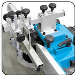
Guide with horizontal and vertical pressers
